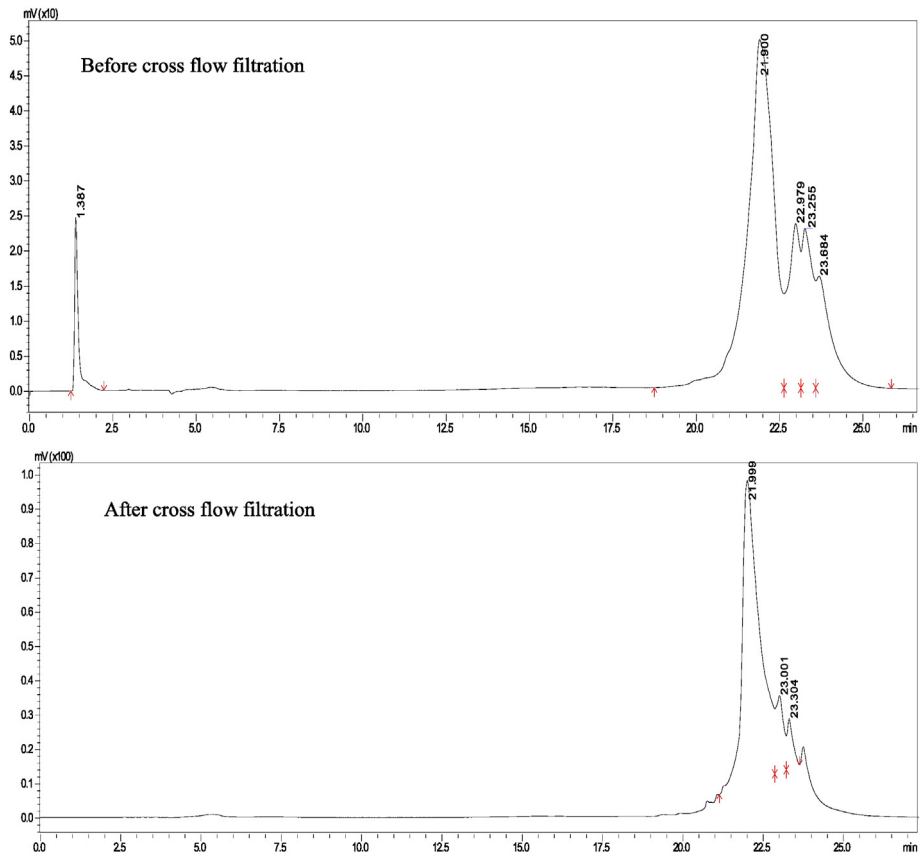
Fig. 3. RP-HPLC profiles of cell lysate before and after cross flow filtration. The maximum purity of rhAT ( \geq 94\% ) was achieved with temperature ( 22^{\circ}\text{C} ) and transmembrane pressure (16 psi).
