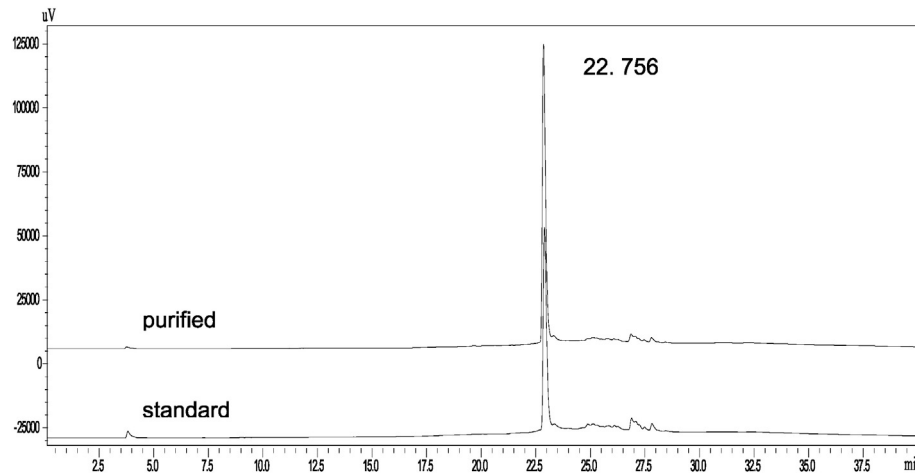
Fig. 5. RP-HPLC analysis of purified rhAT eluted through a phenomenex C-18 column (250 × 4.6 mm) column. The peaks were auto scaled according to the largest intensity peak. The maximum purity of the rhAT ( \geq 98\% ) was observed with retention time 22.756 min.
