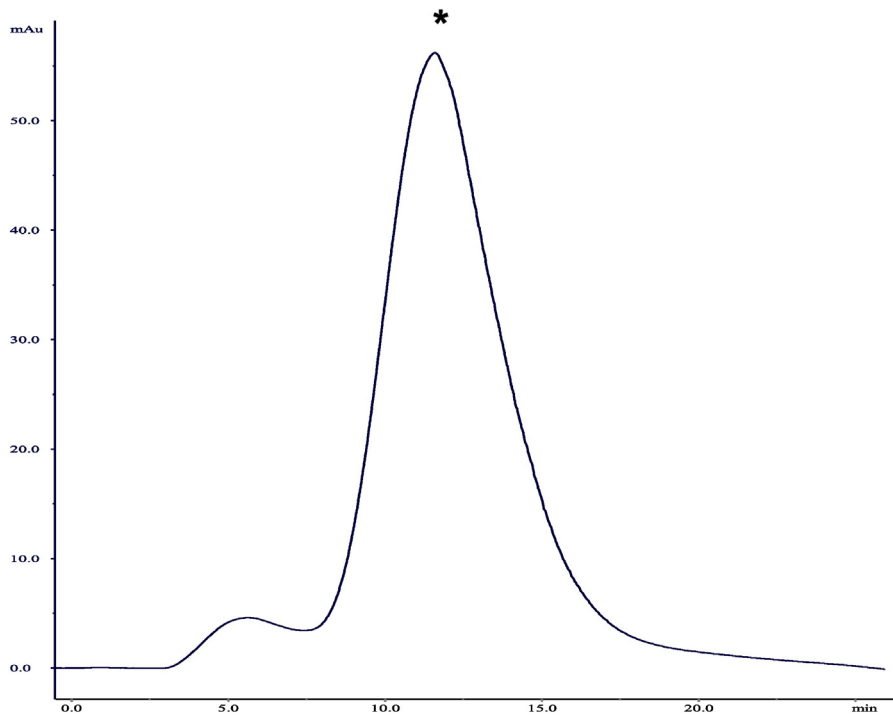
Fig. 4. FPLC chromatogram of rhAT eluted through the IEC with SP-Sepharose FF resin. Monomer peak (indicated with *) of rhAT with a good resolution was separated with maximum recovery yield and purity of 55 and \geq 98\% , respectively.
