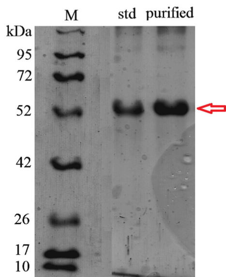
Fig. 8. SDS-PAGE analysis of purified rhAT. Lane M protein molecular weight marker, lane 1 rhAT reference standard and, lane 2 purified rhAT.
