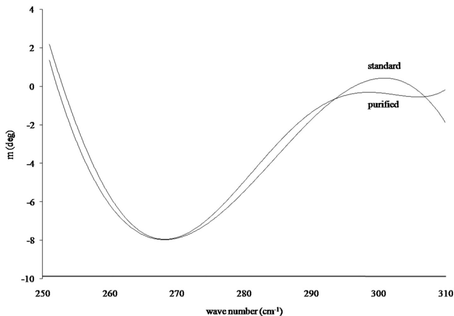
Fig. 6. Secondary structure analysis of rhAT by CD spectroscopy. The CD spectra of both the standard and purified rhAT were shown as \alpha -helix (32%), \beta -sheet (16%), beta turns (10%), and random coil form (6%) of polypeptide chain components.
