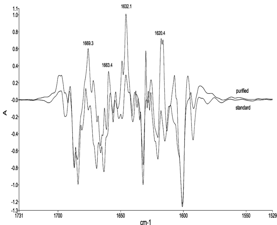
Fig. 7. FT-IR absorbance spectra of the purified and reference standard rhAT. Spectra shows the amide I and II bands, which are the backbone of the protein polypeptide chain. The secondary structural components of amide I region consists of \alpha -helix ( 1663 \pm 2 \text{ cm}^{-1} ) and \beta -sheet ( 1669 \pm 2 \text{ cm}^{-1} ).
