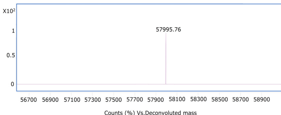
Fig. 10. LC-MS analysis of rhAT. Molecular mass of rhAT (57,995.36 Da) was matched with the antithrombin molecular weight, which is confirmed by the Bioconfirm software.
