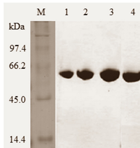
Fig. 2. Native PAGE analysis of rhAT lysate samples with 5 and 10 mL of lysis buffer. Lanes 1 and 2 show the rhAT test samples. Lanes 3 and 4 show control AT samples. Similar antithrombin (58 kDa) bands were observed with respect to different volumes of lysis buffer volumes (5 and 10 mL) and the molecular weight of both purified and control antithrombin (58 kDa) was compared with molecular weight marker (lane M).
