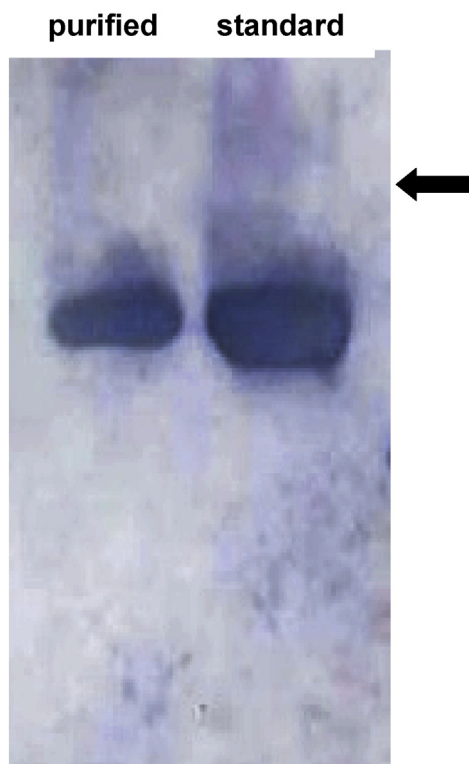
Fig. 9. Western blot analysis of the purified rhAT with a reference standard. Lane 1 shows the purified rhAT. Lane 2 shows standard rhAT. Western blot analysis of rhAT was performed using polyclonal antibody generated from the rabbits and horseradish peroxidase (HRPO)-conjugated goat anti rabbit IgG antibody.
